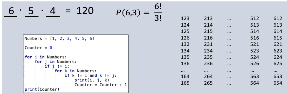
Figure 2. “How many three-digit sequences can be made from the numbers 1-6 that have no repeated digits?”
